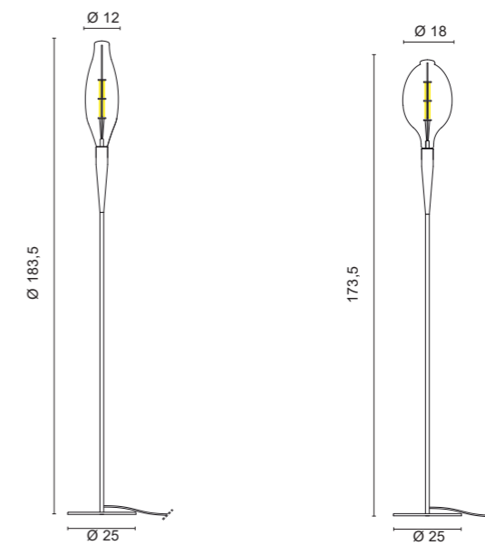
3511 .70 Retro' Accensione ON-OFF ON-OFF switch Light sources E27 LED 11W 2000K 1000lm ▽ 4,30 Kg
